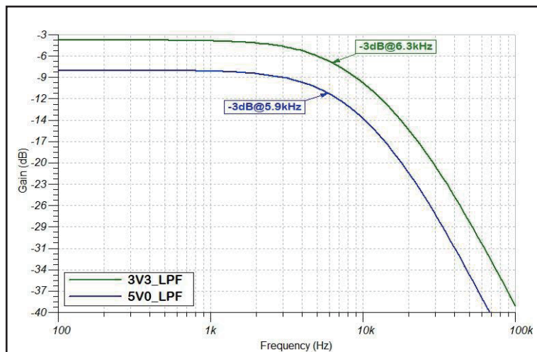
PWM Low-Pass filter for 3.3 V and 5 V logic levels
